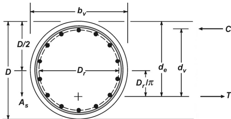
Figure 6.11. Illustrations of terms b_v , d_v , and d_e for circular sections (AASHTO 2012)
