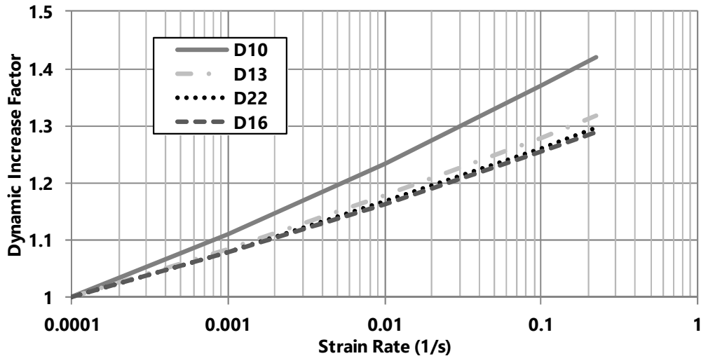
Figure 4.8. Dynamic increase factor due to strain rate effects
