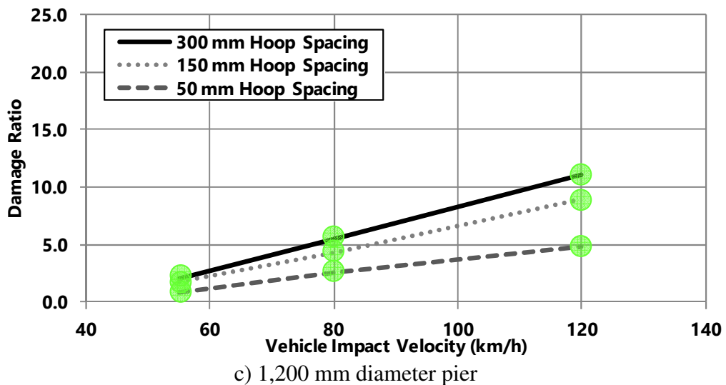
Figure 6.41. Damage ratio vs. vehicle impact velocity for different pier diameters
